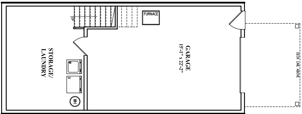
Basement Plan
