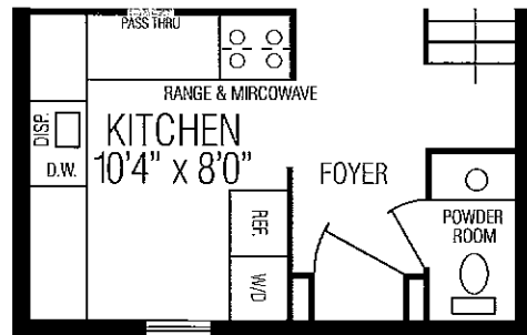
Alternative Kitchen Floor Plan
