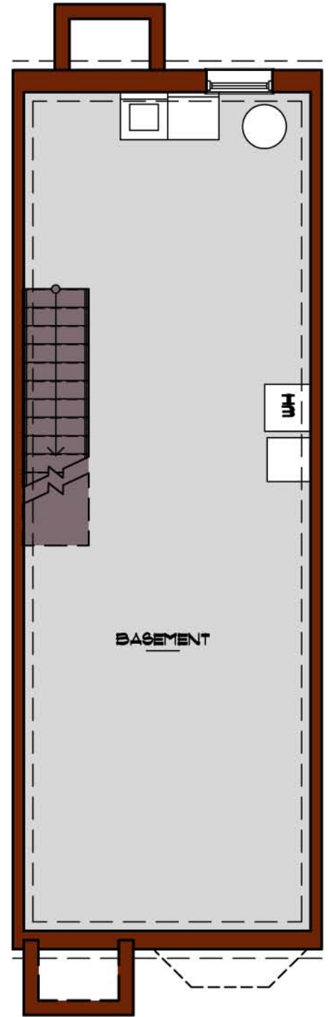
Basement
