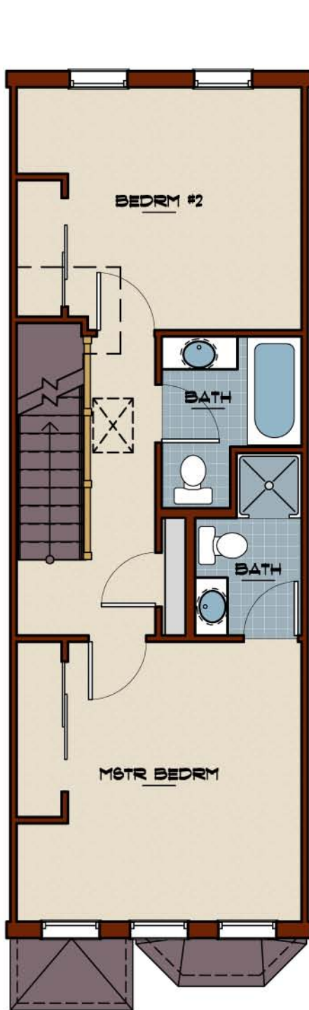
Floor 2
